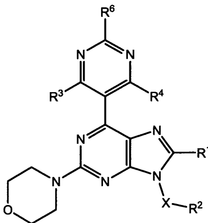
Formula (Ib)
