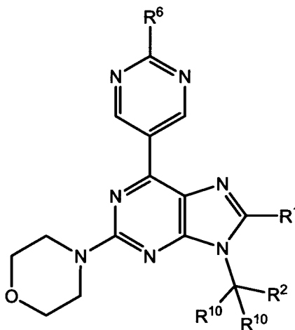
Formula (III)
