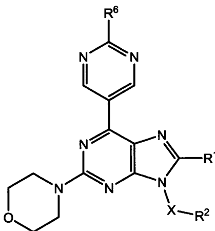
Formula (Ic)
