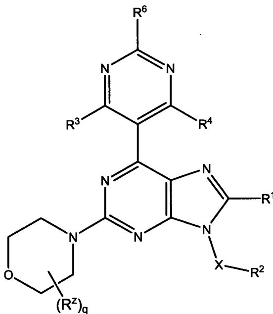
Formula (I)
