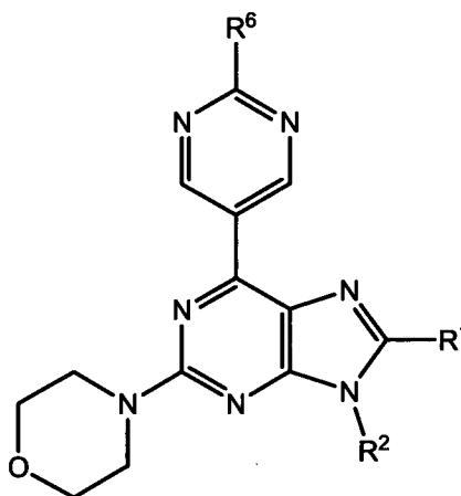
Formula (II)
