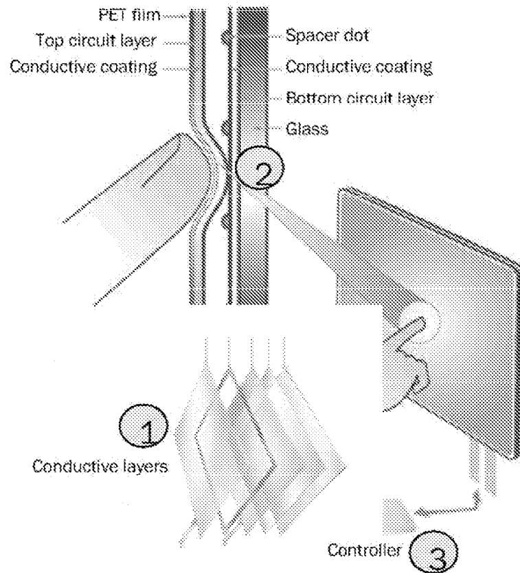
FIG. 2 (PRIOR ART)
