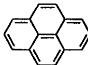
Pyrene*
