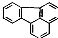
Fluoranthene
