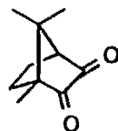
(1R)-(-)-Camphorquinone
