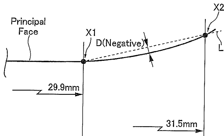
SKI JUMP SHAPE
