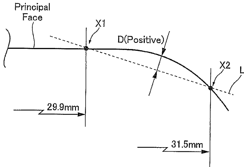
ROLL-OFF SHAPE
