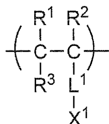
Formula (B2)
