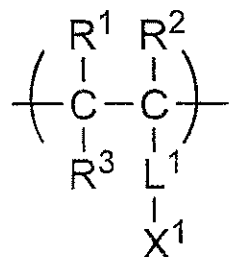
Formula (B2)
