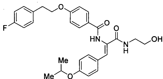
(73a) N-{4-[2-(4-Fluorophenyl)ethoxy]benzoyl}glycine
