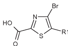
4-Bromo-thiazole-2-carboxylic acid
