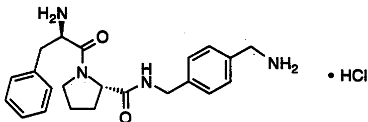
D-Phe-Pro-p-NHCH 2 C 6 H 4 CH 2 NH 2 · HCl
