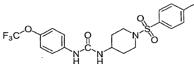
1-[1-(Toluene-4-sulfonyl)-piperidin-4-yl]-3-(4-trifluoromethoxy-phenyl)-urea (1711)
