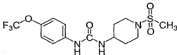
1-(1-Methanesulfonyl-piperidin-4-yl)-3-(4-trifluoromethoxy-phenyl)-urea (1709)
