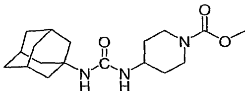
4-(3-Adamantan-1-yl-ureido)-piperidine-1-carboxylic acid methyl ester (1702)
