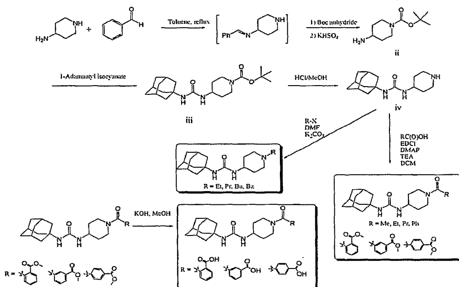
Scheme 1: Synthesis of N-(1-benzoylpiperidin-4-yl)-N'-(adamant-1-yl)ureas.
