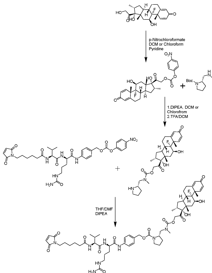
Scheme 10 - Synthetic Scheme for Maleimide-CathepsinBCleavable-Dicarbamate-Dex
