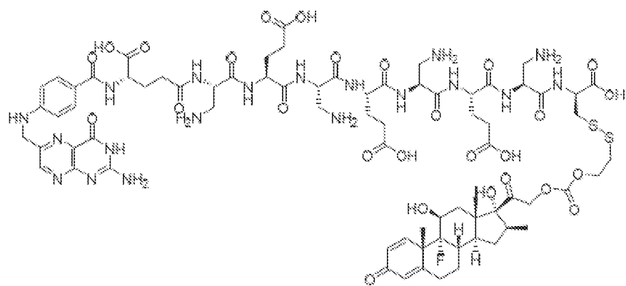
Compound 102:
