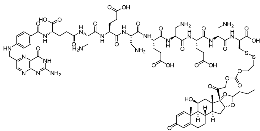
Compound 105:
