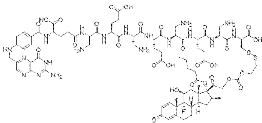
Compound 105:
