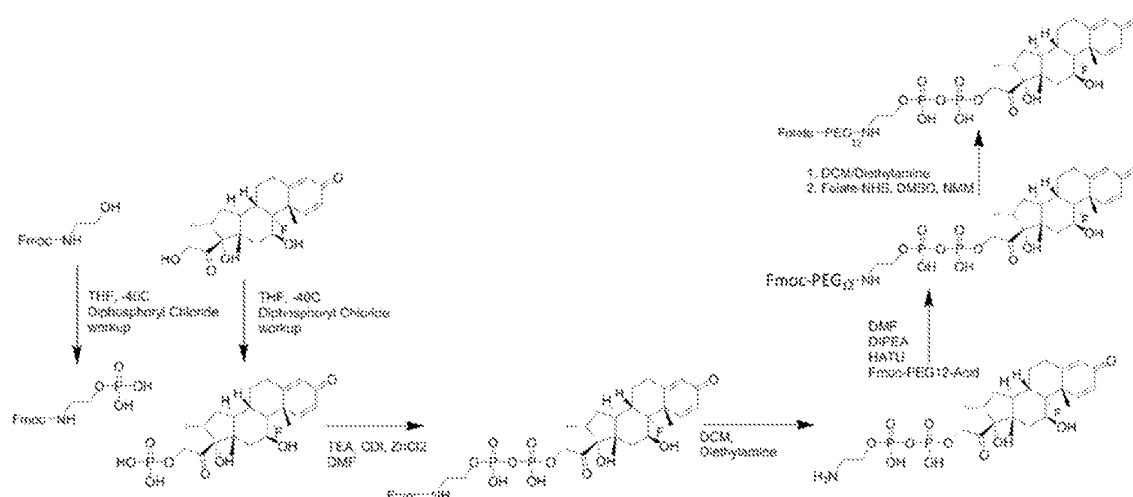
Scheme 12 - Synthetic Scheme of Compound 108 (Folate-PEG12(CH 2 )-Pyrophosphate-Dexamethasone)
