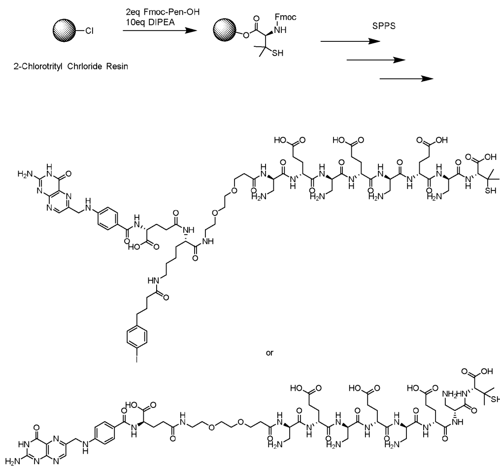
Scheme 6 - Synthetic Scheme of Steroid-Carbamate-Pyridyl Disulfide Compounds
