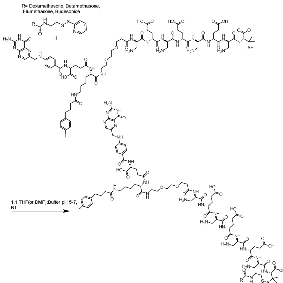
Scheme 8 Final DimethylCys-Maleimide Coupling of Compounds.
