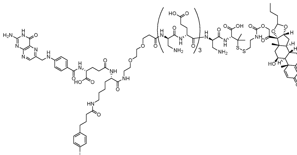
Compound 127 (Folate-AlbuminBinder-PEG2-Hydrolink-DimethylCysteine-Carbamate-Budesonide)
