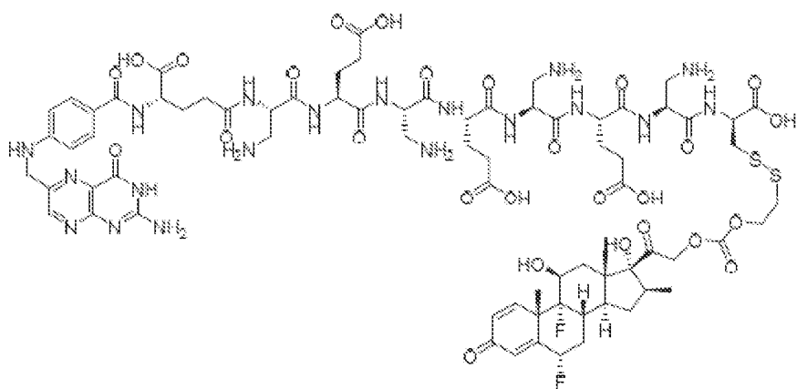
Compound 104:
