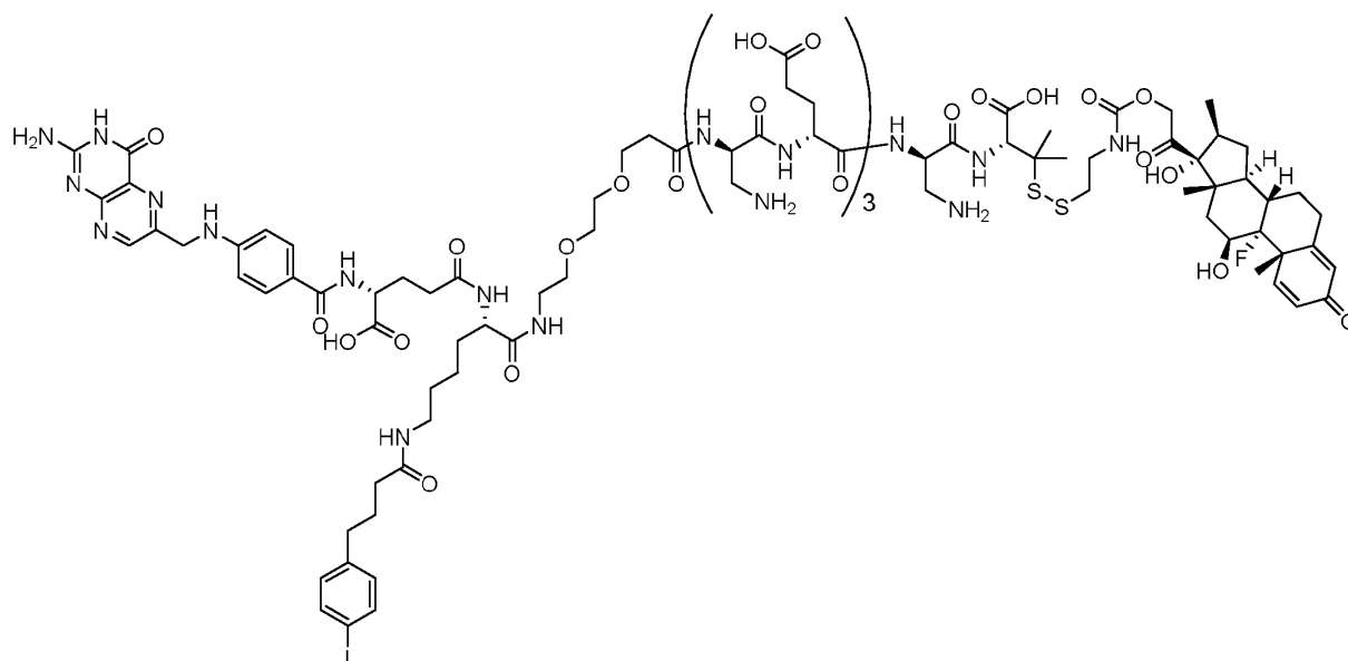
Compound 126 (Folate-AlbuminBinder-PEG2-Hydrolink-DimethylCysteine-Carbamate-Betamethasone)
