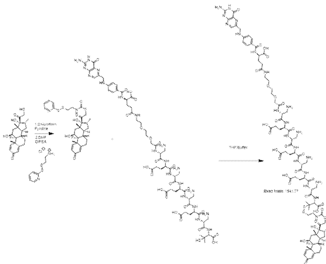
Scheme 9 – Synthetic scheme for Folate-PEG2-Hydrolink-DimethylCysteine-Carbamate-Dexamethasone (Compound 106)
