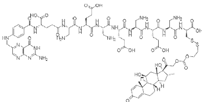
Compound 102:
