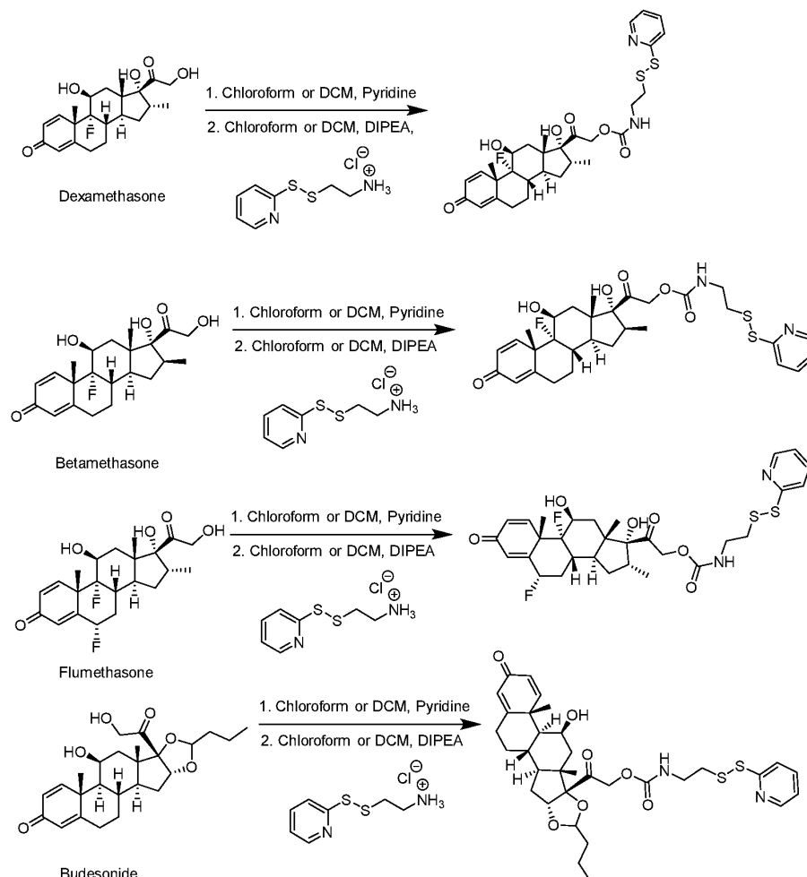
Scheme 7 - Synthetic Scheme of Steroid-Carbamate-Pyridyl Disulfide Compounds
