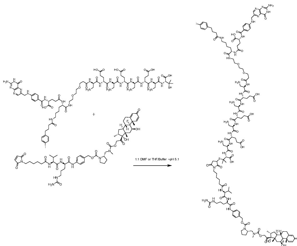
Scheme 11 - Synthesis of Compound 125 (Fol-Alb-PEG2-Hydrolink-DimethylCysteine-Maleimide-(CH 2 ) 5 -CathepsinBCleavable-Dicarbamate-Dexamethasone)
