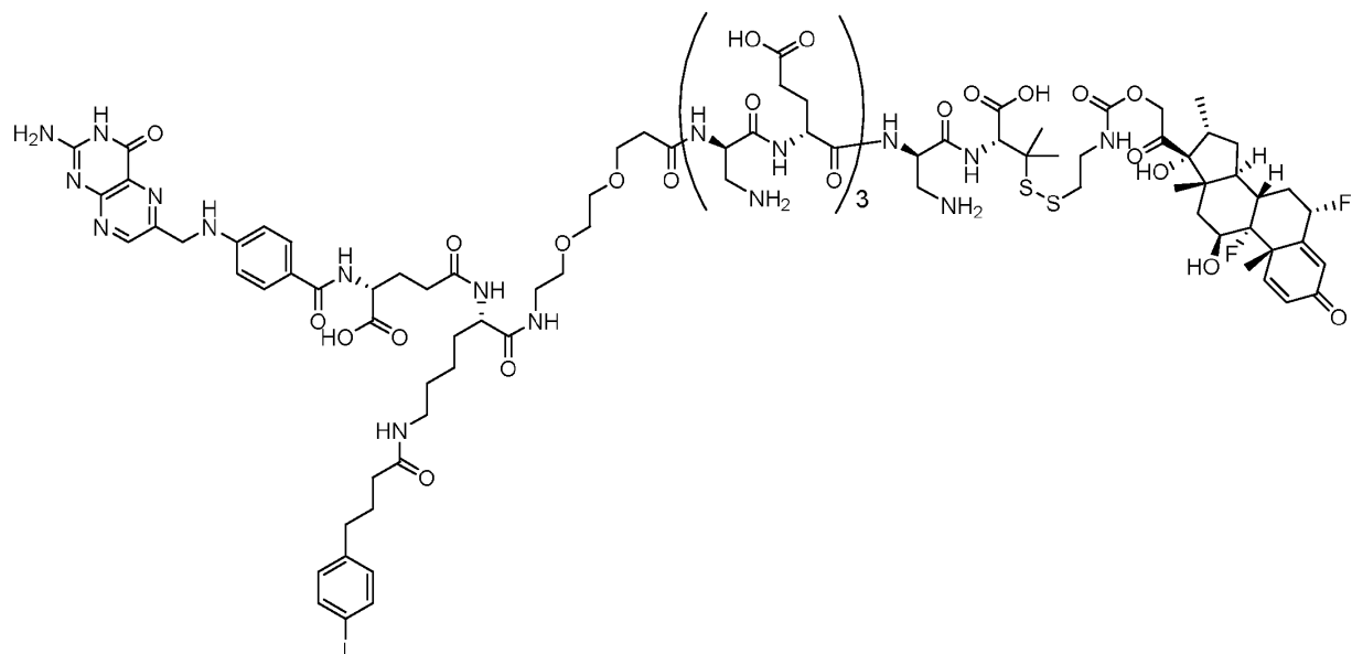
Compound 124 (Folate-AlbuminBinder-PEG2-Hydrolink-DimethylCysteine-Carbamate-Flumethasone)
