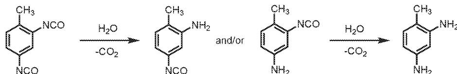
Scheme 1: Effects of water on isocyanate groups of TDI.
