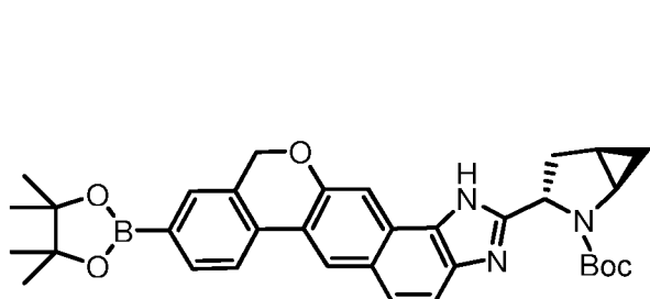
(1R,3S,5R)-tert-butyl 3-(9-(4,4,5,5-tetramethyl-1,3,2-dioxaborolan-2-yl)-1,11-dihydroisochromeno[4',3':6,7]naphtho[1,2-d]imidazol-2-yl)-2-azabicyclo[3.1.0]hexane-2-carboxylate
