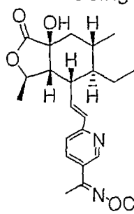
Ex. 13-2: HRMS: 387.2300 ( \text{MH}^+ )
