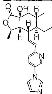
Ex. 13-2: HRMS: 387.2300 ( \text{MH}^+ )
