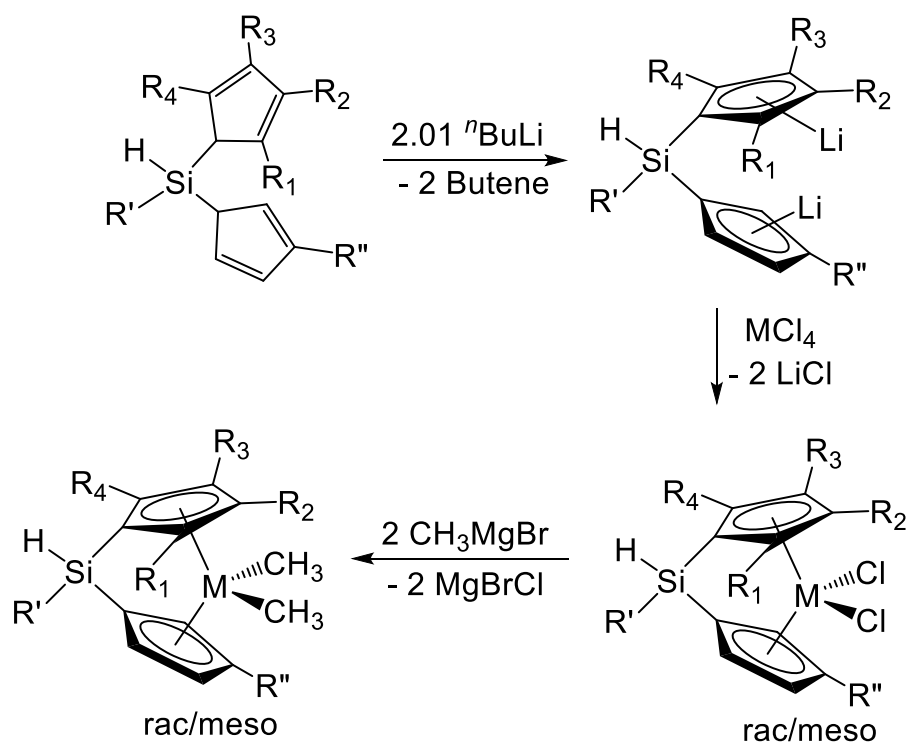
Scheme 2. General synthetic route for Si(H)-bridged metallocenes (where M = \text{Hf, Zr} ; R' = \text{Me, Ph} ; R'' = \text{n-Pr, -CH}_2\text{SiMe}_3 ; R_1 = R_3 = R_4 = \text{Me, H} ; R_2 = \text{Me, n-Pr, -CH}_2\text{SiMe}_3 ).
