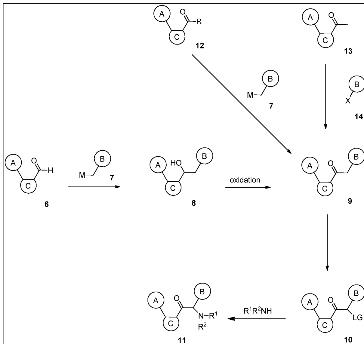
5 Scheme 2: all A, B, C, R 1 , R 2 and LG are as described for the compounds of the present invention according to formula (A) wherein cycle C has a structure as formula (a1) and its embodiments and formulae.
