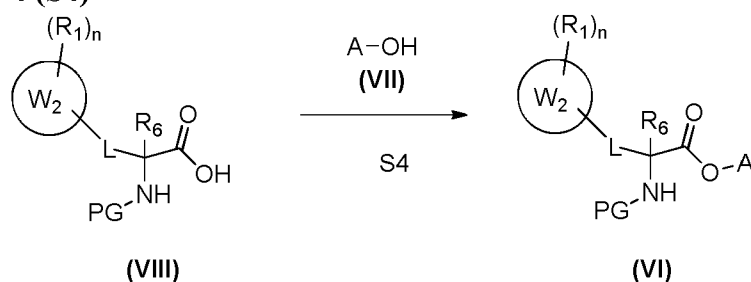
Scheme 4 (S4)
