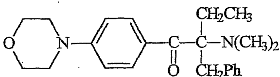
2-benzyl-2-N,N-dimethylamino -1-(4-morpholinophenyl)-1-butanone
