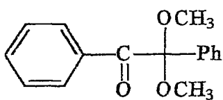
2,2-dimethoxy-2-phenyl acetophenone
