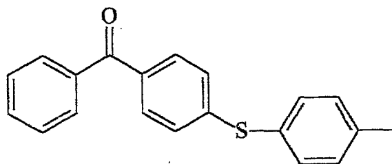
[4-(4-methylphenylthio)phenyl]phenylketone
