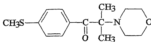
2-methyl-1-[4-(methylthio)phenyl]-2-morpholino propan-1-one
