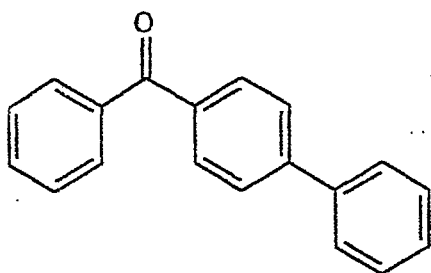
4-phenyl benzophenone
