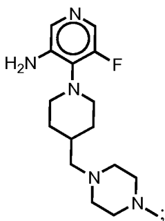
5-fluoro-4-(4-methyl-1-oxa-4,9-diazaspiro[5.5]undecan-9-yl)pyridin-3-amine:
