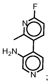
6-fluoro-2-methyl-[3,4'-bipyridin]-3'-amine:
