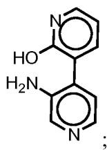
4-(4-methylpyridazin-3-yl)pyridin-3-amine:
