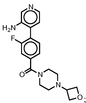
(3'-amino-[3,4'-bipyridin]-6-yl)(4-(oxetan-3-yl)piperazin-1-yl)methanone:
