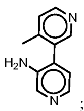
4-(3-methylpyridazin-4-yl)pyridin-3-amine:
