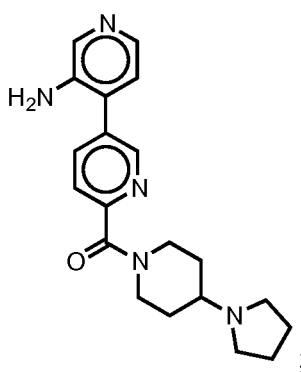
(3'-amino-[3,4'-bipyridin]-6-yl)(4-(azetidin-1-yl)piperidin-1-yl)methanone:
