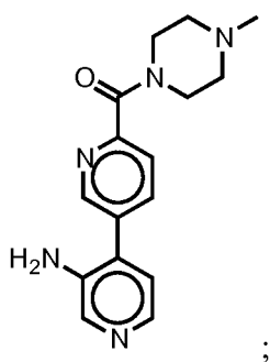
6-(4-methylpiperazin-1-yl)-[3,4'-bipyridin]-3'-amine:
