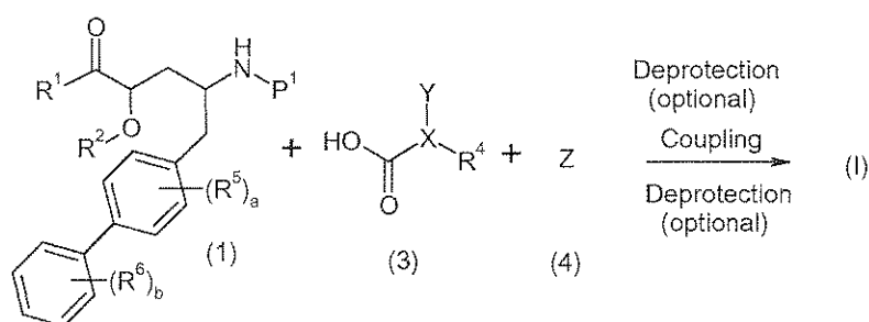
Scheme II
