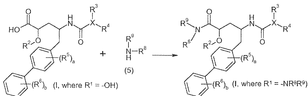
Scheme III
