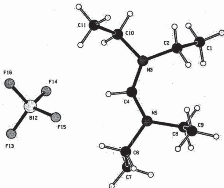
Figure 2: N,N,N'-Tetraethylformamidineium tetrafluoroborate
