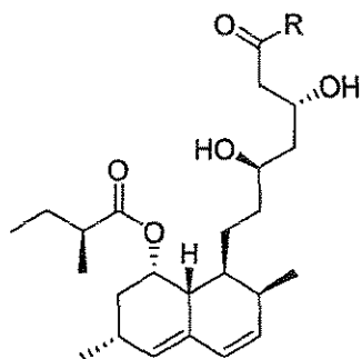
Lovastatin acid, amide or ester
