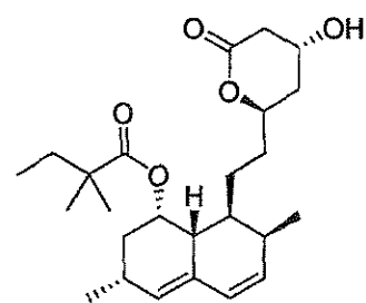
Simvastatin lactone
