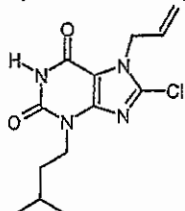
a) 8-chloro-3-(3-methylbutyl)-7-(2-propen-1-yl)-3,7-dihydro-1H-purine-2,6-dione
