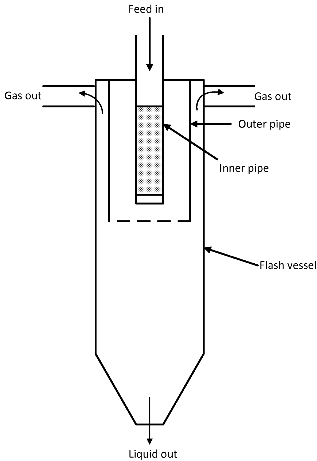
Figure 1, Flash separator
