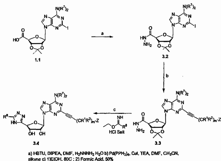
Scheme 3: Preparation of 4' triazoles:
