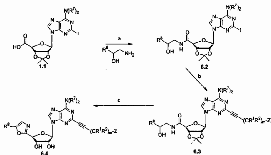
Scheme 6: Preparation of 4'-1,3 oxazole
