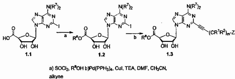
Scheme 1: Preparation of 5' ester analogs:
