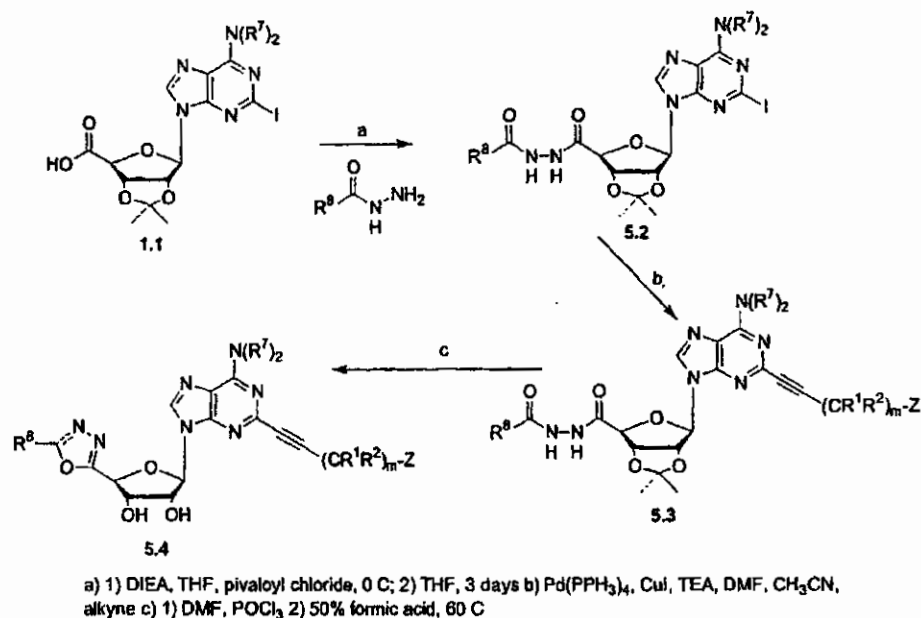
Scheme 5: Preparation of 4'-1,3,4 oxadiazoles
