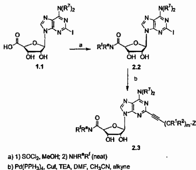
Scheme 2: Preparation of 5' amide analogs:
