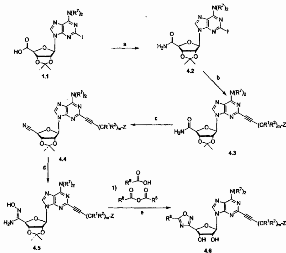
Scheme 4: Preparation of 4'-1,2,4-oxadiazoles
