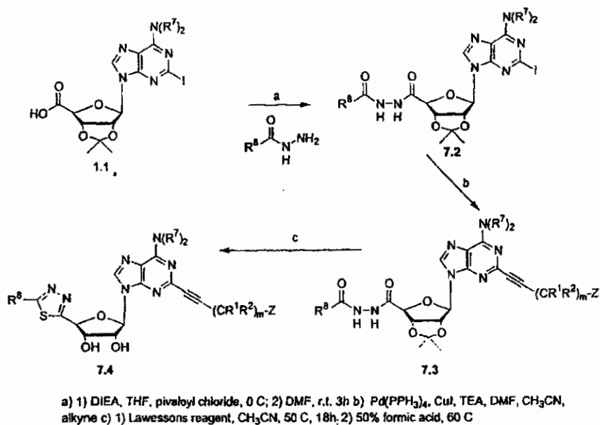
Scheme 7: Preparation of 4'-1,3,4 thiadiazole
