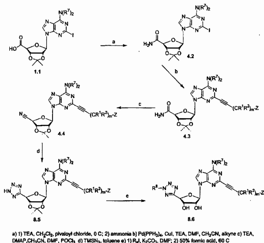
Scheme 8: Preparation of 4'-tetrazole
