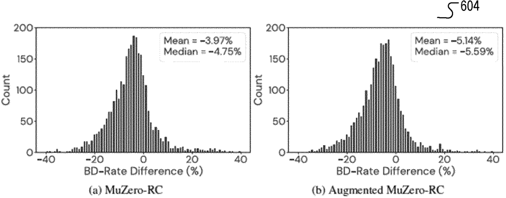
Histogram of SSIM BD-Rate difference of agent compared to libvpx on evaluation set.
