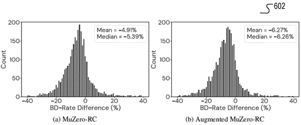
Histogram of PSNR BD-Rate difference of agent compared to libvpx on evaluation set.
