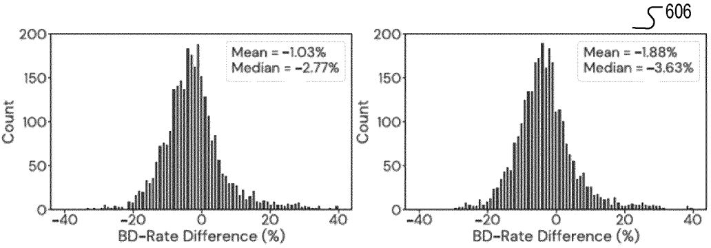
Histogram of VMAF BD-Rate difference of agent compared to libvpx on evaluation set.
