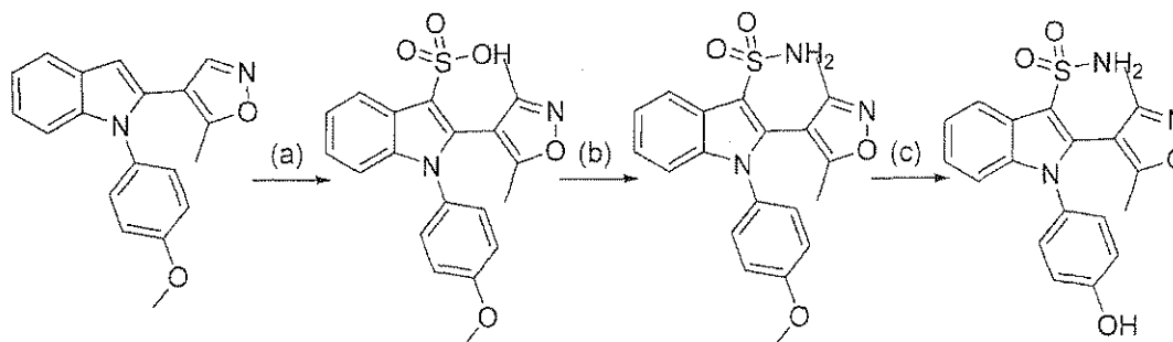
Scheme 39
