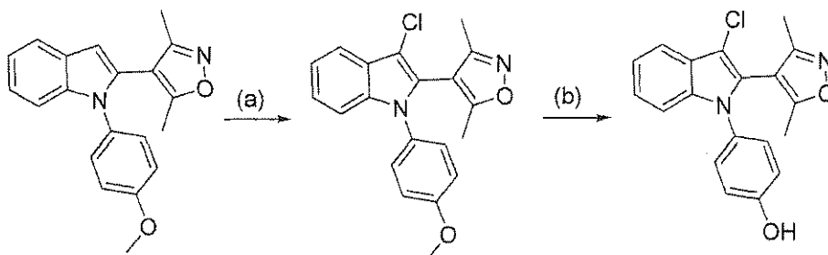
Scheme 38
