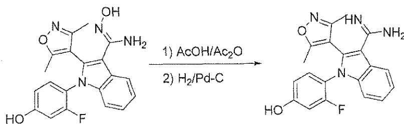
Scheme 40
