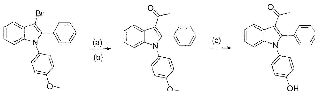
Scheme 8
