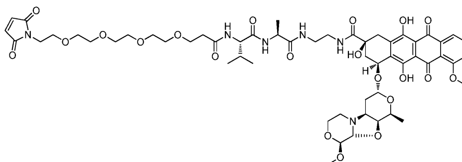
MA-PEG4-va-EDA-PNU159682
