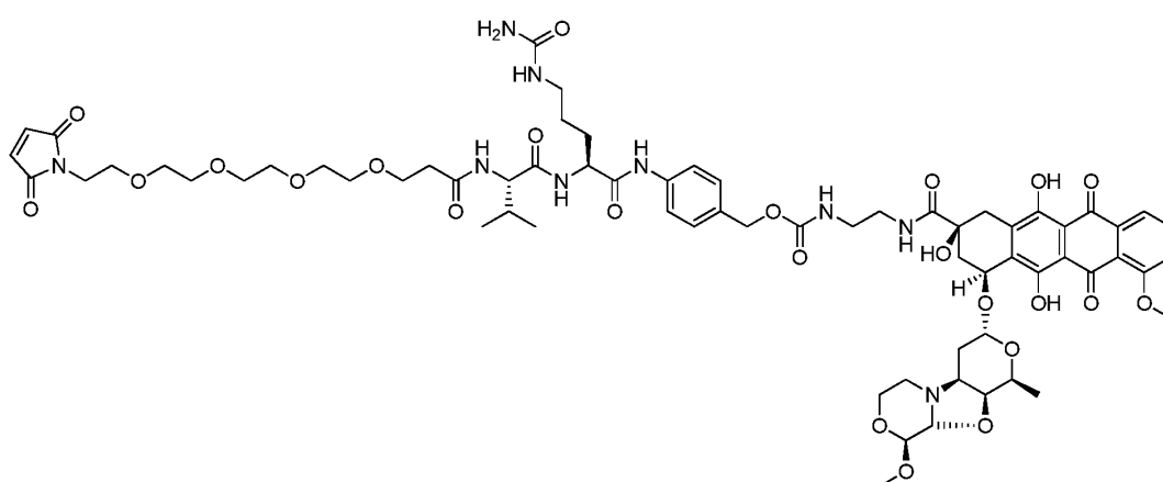
MA-PEG4-vc-PAB-EDA-PNU159682
