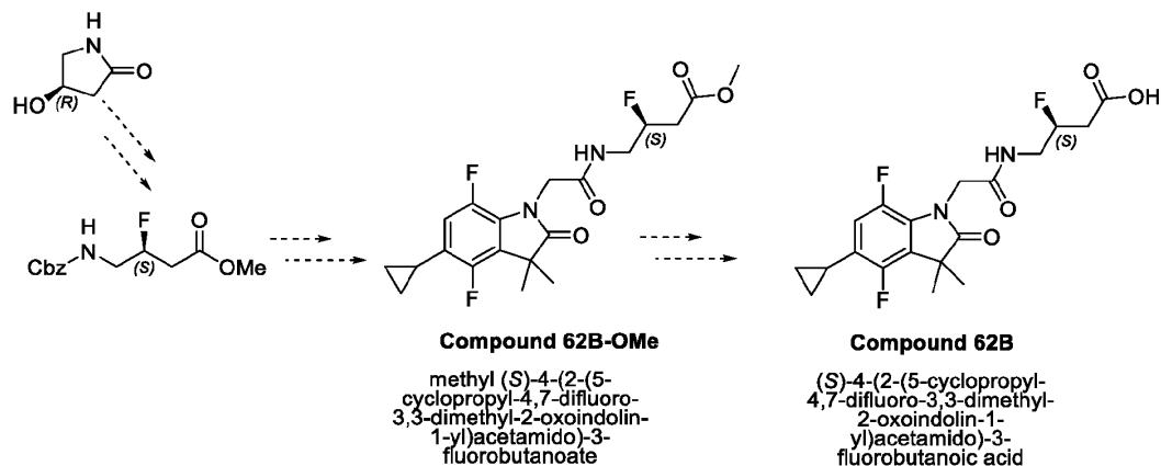
Scheme 19B.
