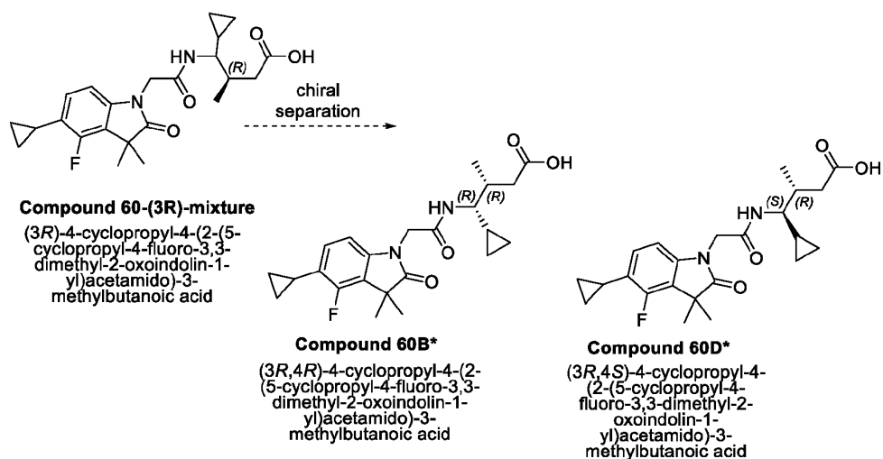
Scheme 17B.
