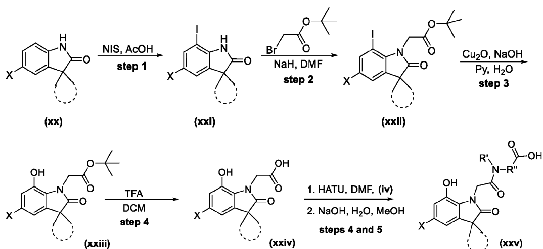
General Scheme 7
