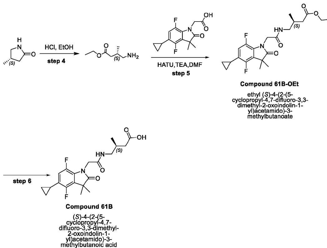
Scheme 18B.
