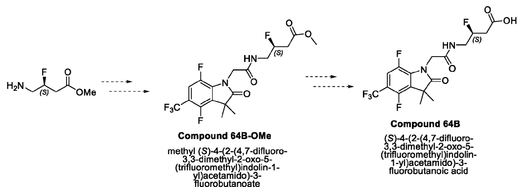
Scheme 21C.
