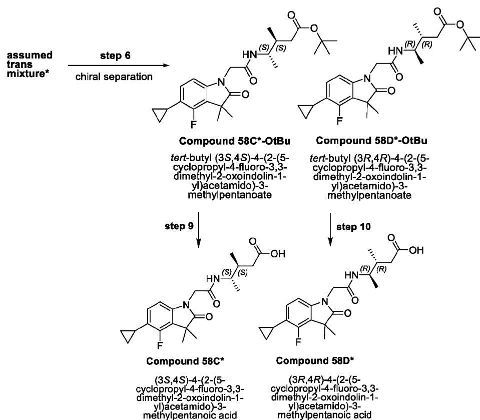
Scheme 15C.
