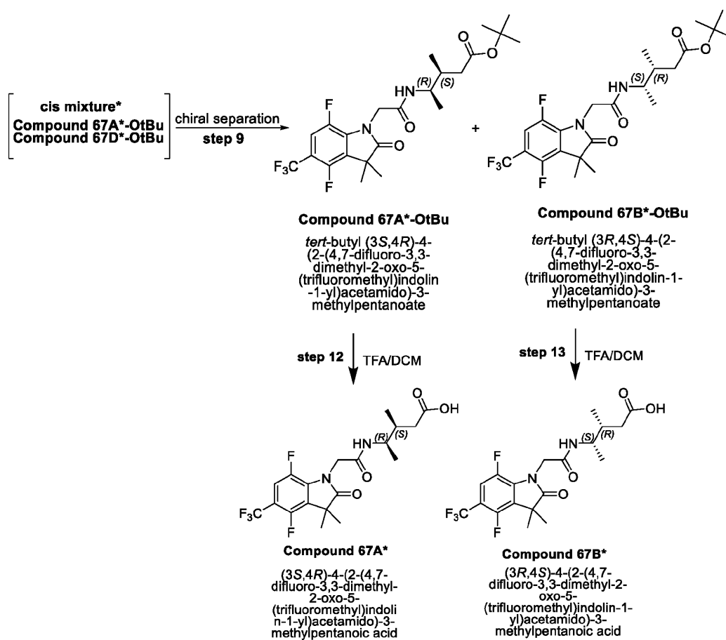
Scheme 23B.
