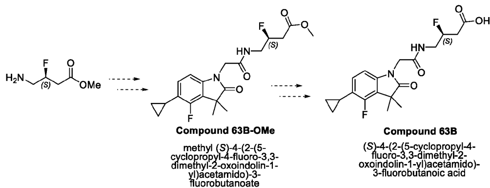
Scheme 20B.
