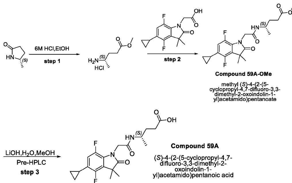
Scheme 16B.
