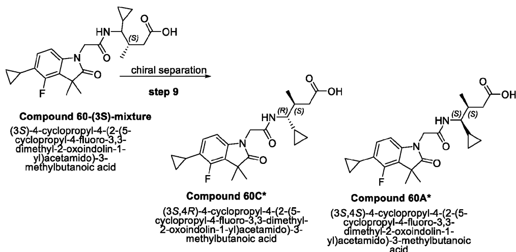
Scheme 17B.
