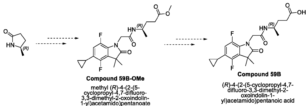
Scheme 16B.
