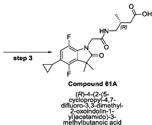
Scheme 18B.
