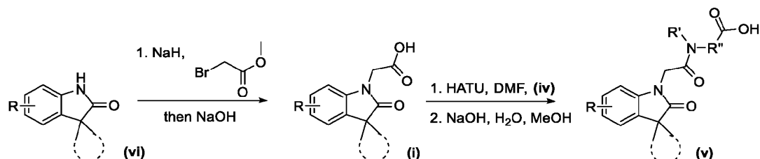
General Scheme 3
