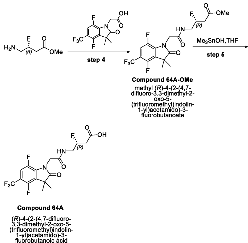
Scheme 21C.
