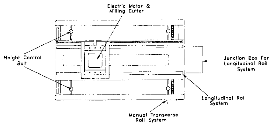
FIGURE 1. IMPROVED PORTABLE MILLER (PLAN VIEW)
