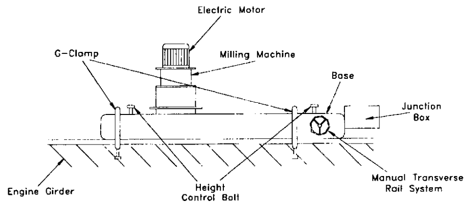
FIGURE 2. IMPROVED PORTABLE MILLER (PROFILE VIEW)
