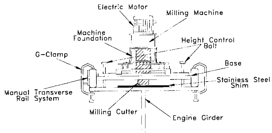
FIGURE 3. IMPROVED PORTABLE MILLER (SIDE VIEW)
