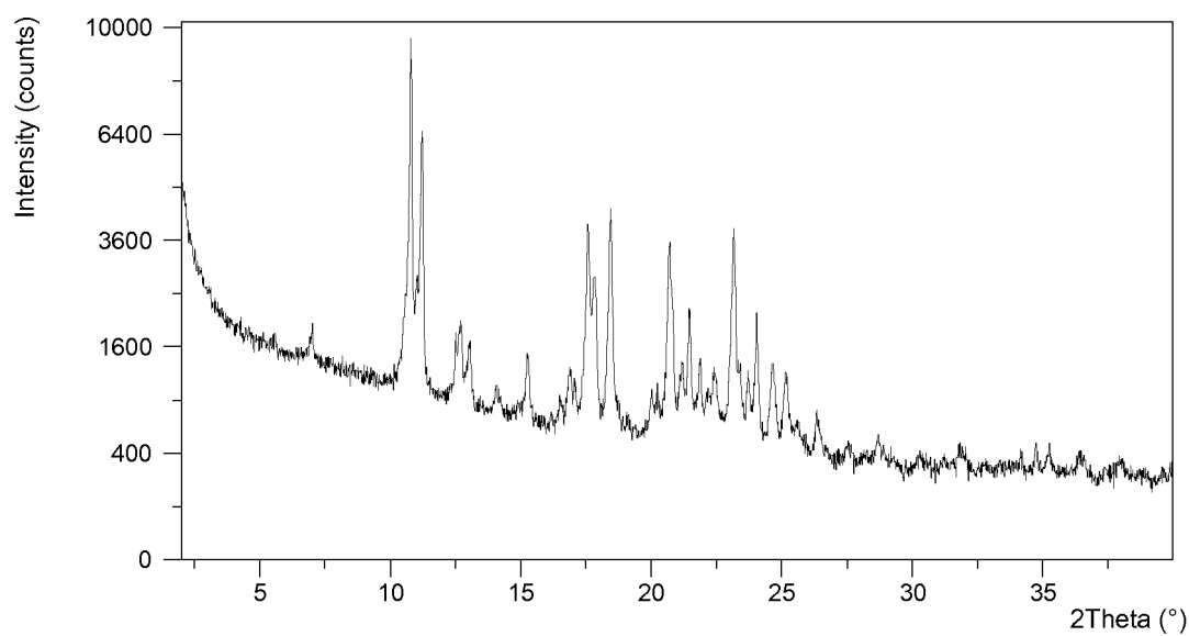
Figure 6. The PXRD pattern of Form 2 of the compound of Formula (I)
