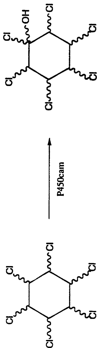
Hexachlorocyclohexane
