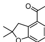
Isomer B
