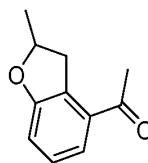
Isomer B
