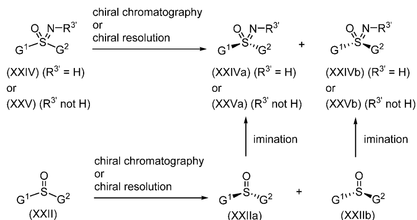
Scheme 11
