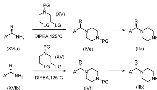
Scheme 7
