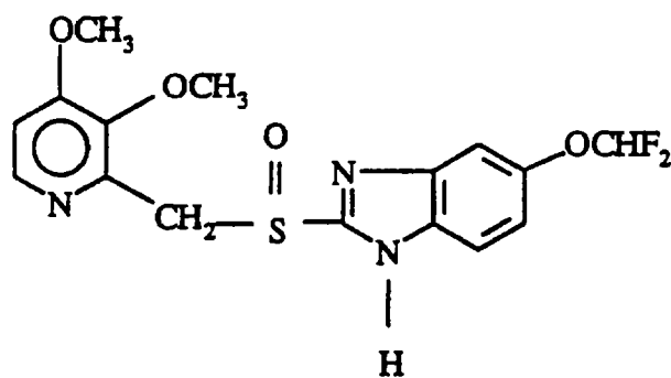
Pantoprazole
