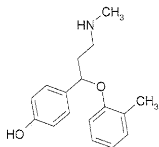
Hydroxylated Metabolite
