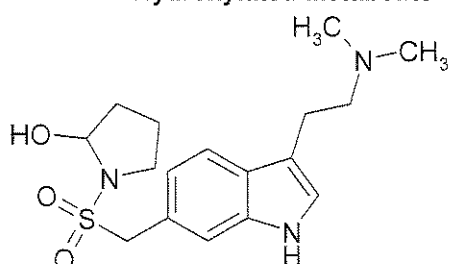
Hydroxylated Metabolite
