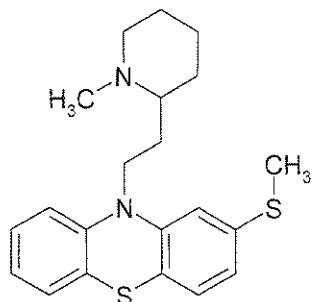
Chemical Structure
