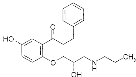
Hydroxylated Metabolite
