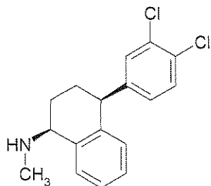
Chemical Structure
