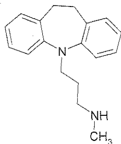
Chemical Structure
