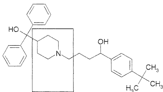
Terfenadine
