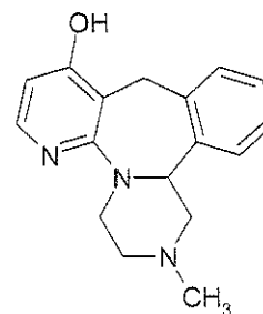
Hydroxylated Metabolite
