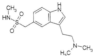
Chemical Structure
