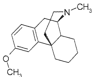
Chemical Structure
