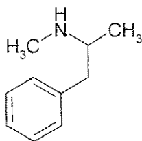
Chemical Structure
