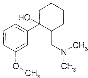
Chemical Structure
