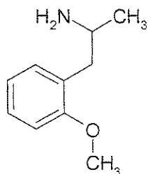
Chemical Structure
