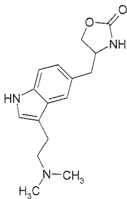
Chemical Structure
