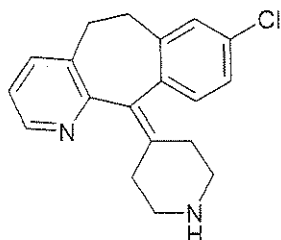
Chemical Structure
