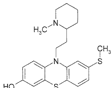
Hydroxylated Metabolite
