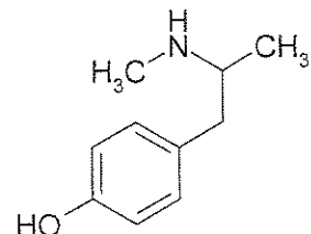
Hydroxylated Metabolite
