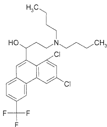
Chemical Structure
