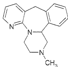
Chemical Structure
