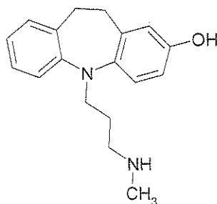
Hydroxylated Metabolite
