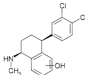
Hydroxylated Metabolite
