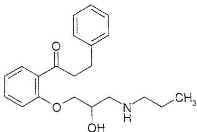
Chemical Structure
