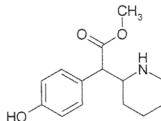
Hydroxylated Metabolite
