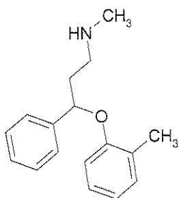
Chemical Structure
