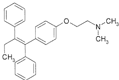
Chemical Structure
