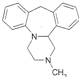
Chemical Structure
