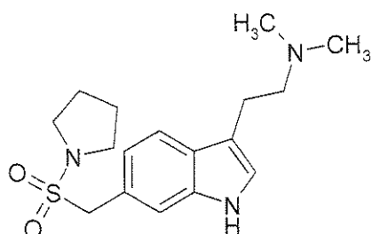
Chemical Structure
