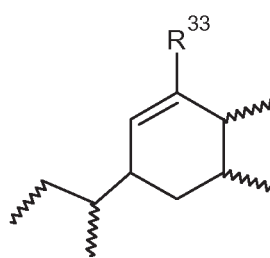
Structure V^c
