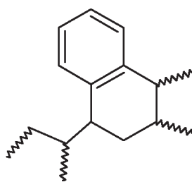
Structure V^b
