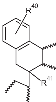
Structure V^h
