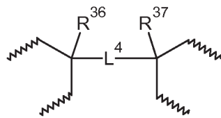
Structure V^b
