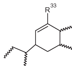
Structure V^c
