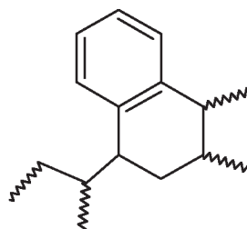
Structure V^b
