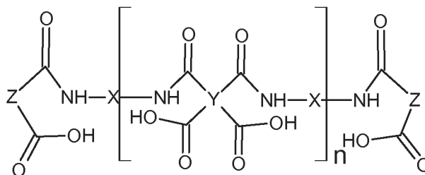
Structure VIII
