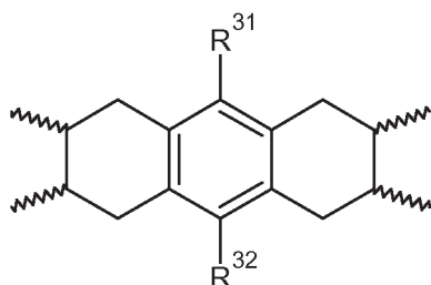
Structure V^a
