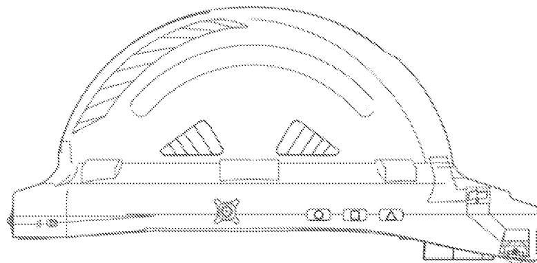
Figure 5: Side view of the variable speed multi directional air ventilation and purification helmet
