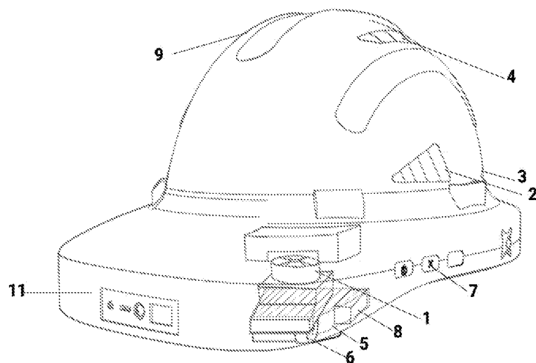
Figure 3: Perspective view of the variable speed multi directional air ventilation and purification helmet
