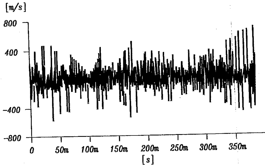
(a) Time Domain Plot
