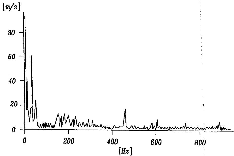
(b) Frequency Domain Plot
