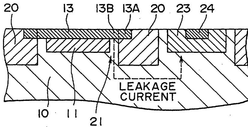
FIG. 3A RELATED ART
