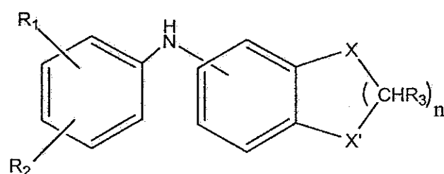
Formula I
