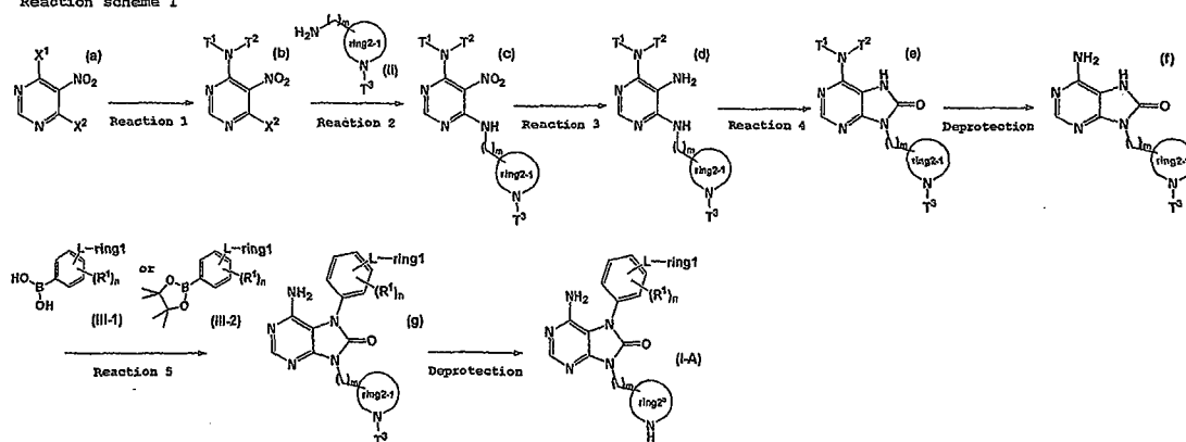
Reaction scheme 1
