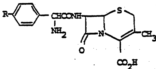
R=H cephalosporin IX
