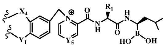
LB39 (Bortezomib analog), wherein Y 5 is N,
