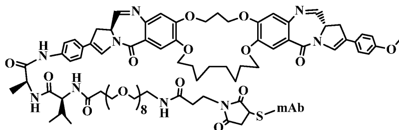
A PBD dimer conjugate, studied by Bristol-Myers Squibb.
