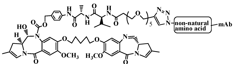
The SG-3199 conjugate, studied by Allozyne, Inc.
