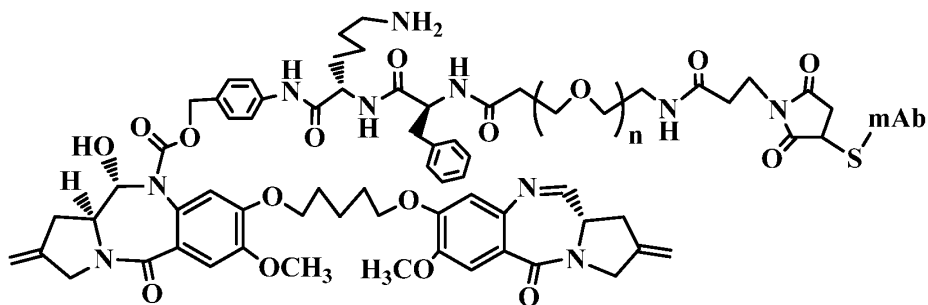
The SG2057 conjugate, used by Genentech Inc.
