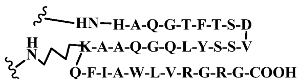
LB44 (Clindamycin),
