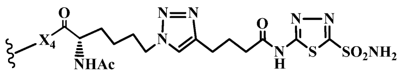
LB10 (CAIX ligand),
