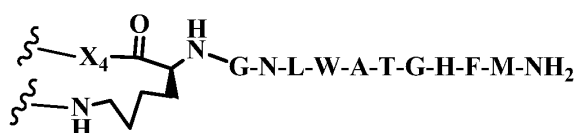
LB20 (Neuromedin B),
