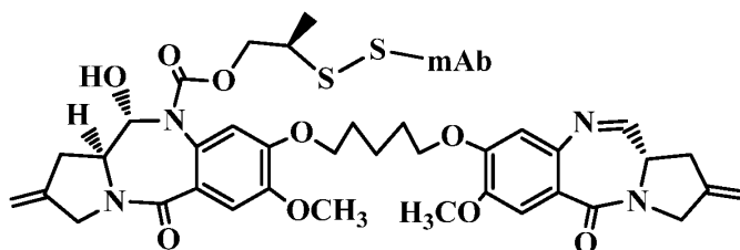
A PBD conjugate via a traceless linker by Genentech Inc
