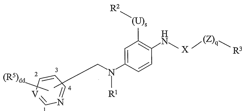
(XXXXIII)
