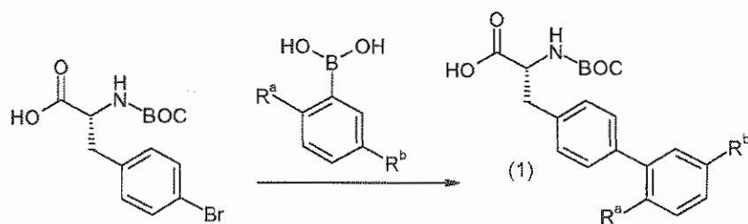
Scheme V
