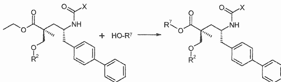
Scheme I
