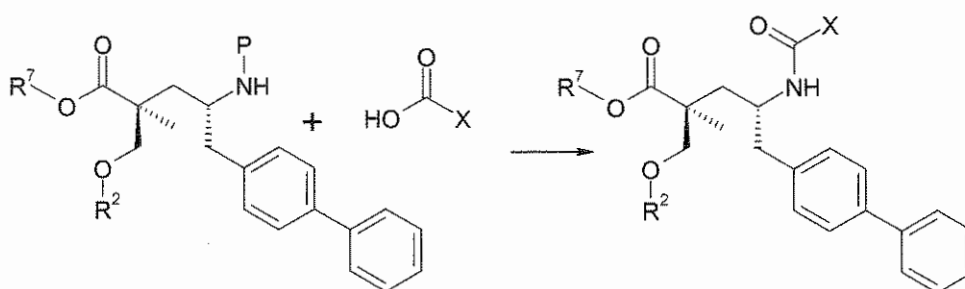
Scheme IV
