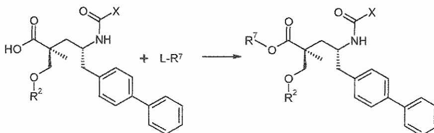
Scheme II
