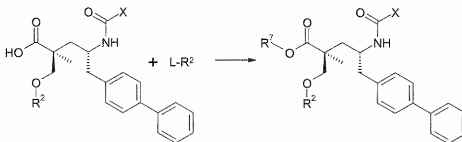
Scheme III
