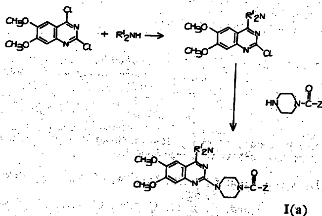
Equation 4.
