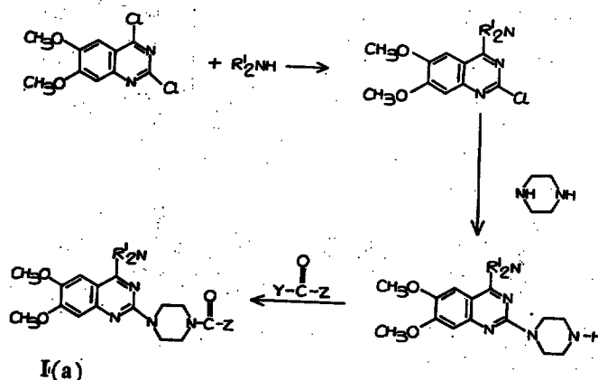
Equation 3.
