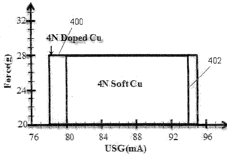
Fig 4(a) - Ball Bond Process Window
