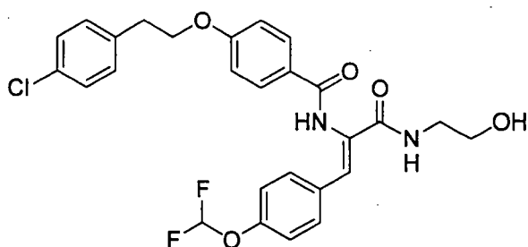
(78a) N-{4-[2-(4-Chlorophenyl)ethoxy]benzoyl}glycine
