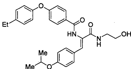
(89a) N-[4-(4-Ethylphenoxy)benzoyl]glycine
