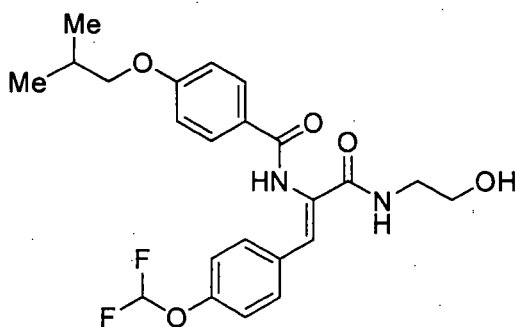
(30a) N-(4-Isobutoxybenzoyl)glycine
