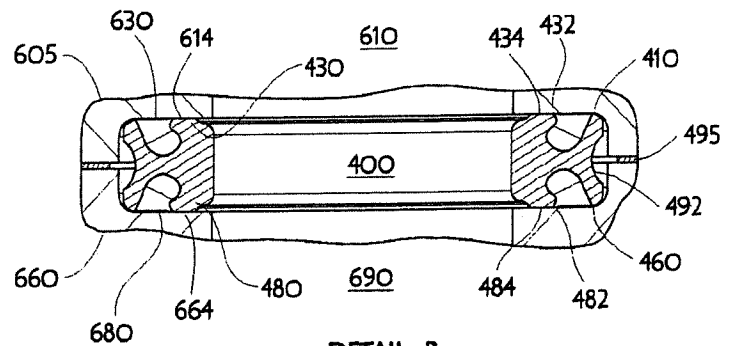
DETAIL B Fig. 6B
