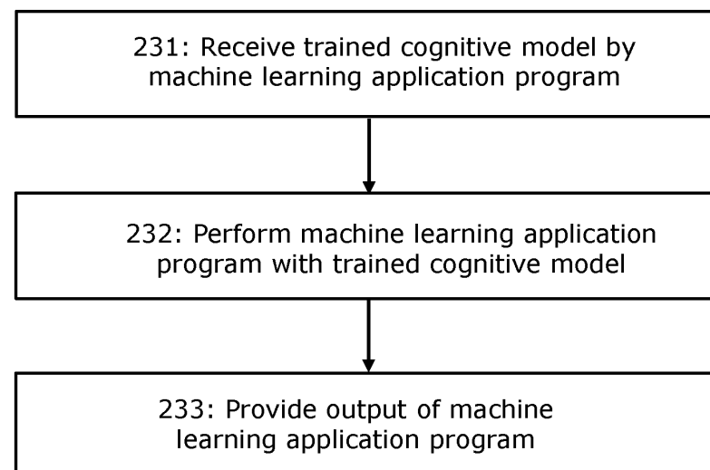
FIG. 2c Inference 230
