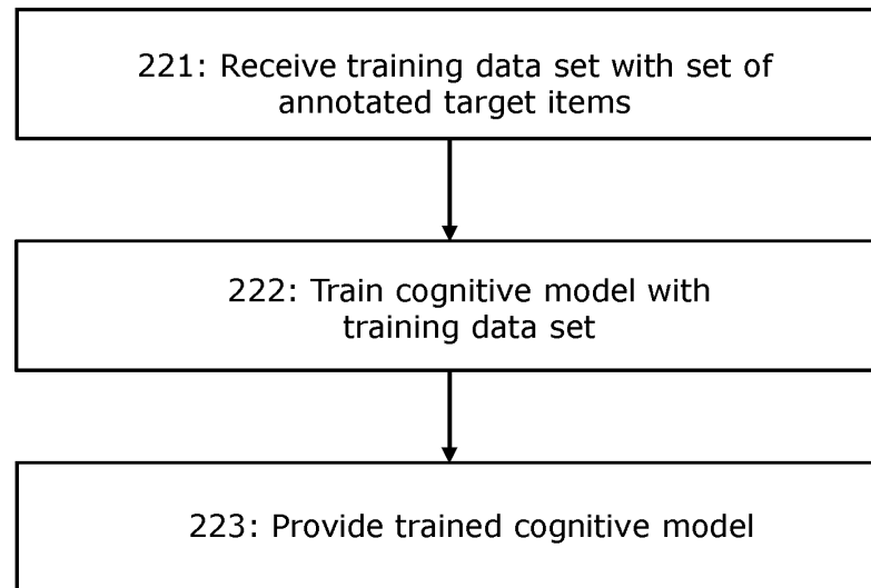
FIG. 2b Training
