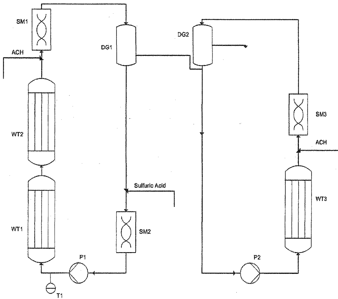
Fig. 2 Flow diagram for comparative examples 1-4
