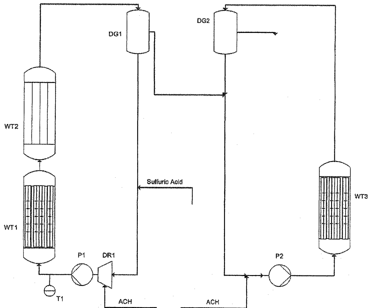
Fig. 3: Flow diagram for examples 1-4
